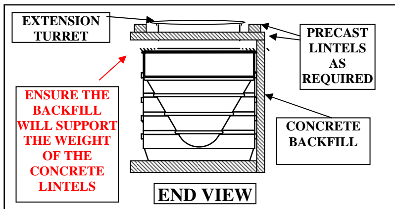
Fig 2: Position of concrete lintels
